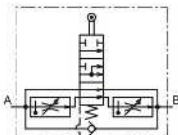
UCF2G-03-※-E-10 UCF2G-04-30-30
