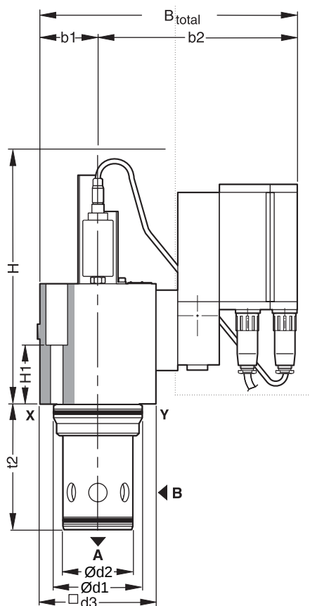
NG50-63
