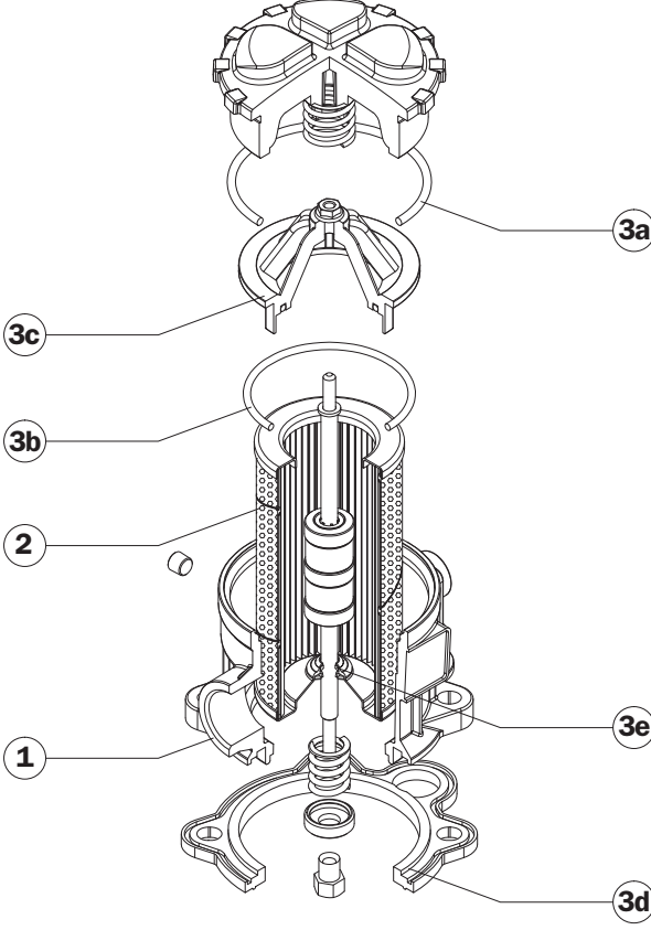
MPH 104 SO
