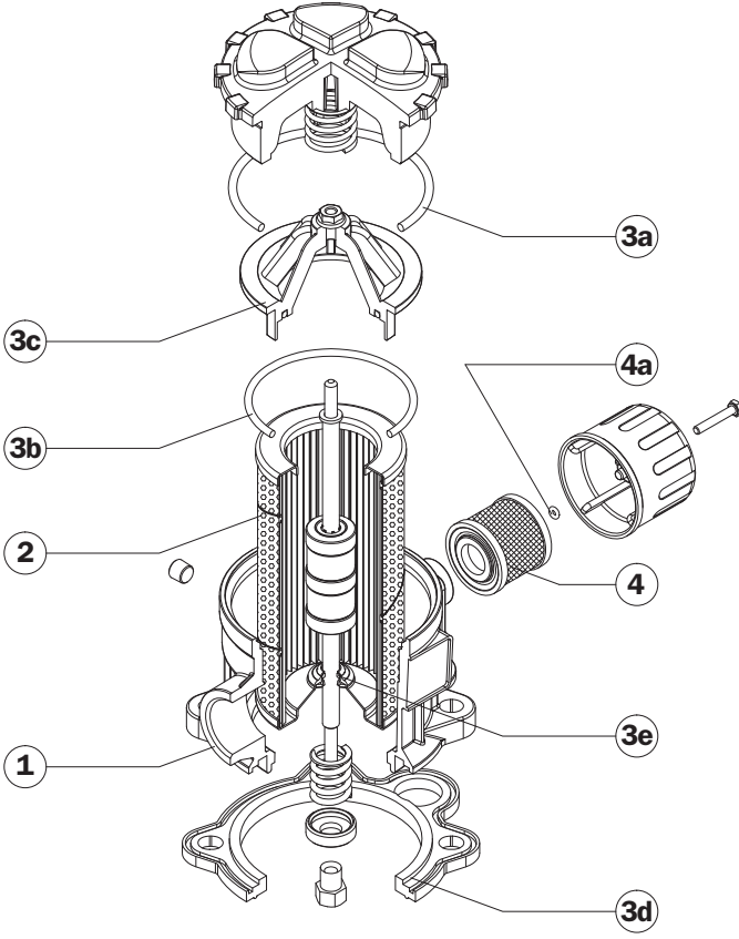
MPH 104 CO
