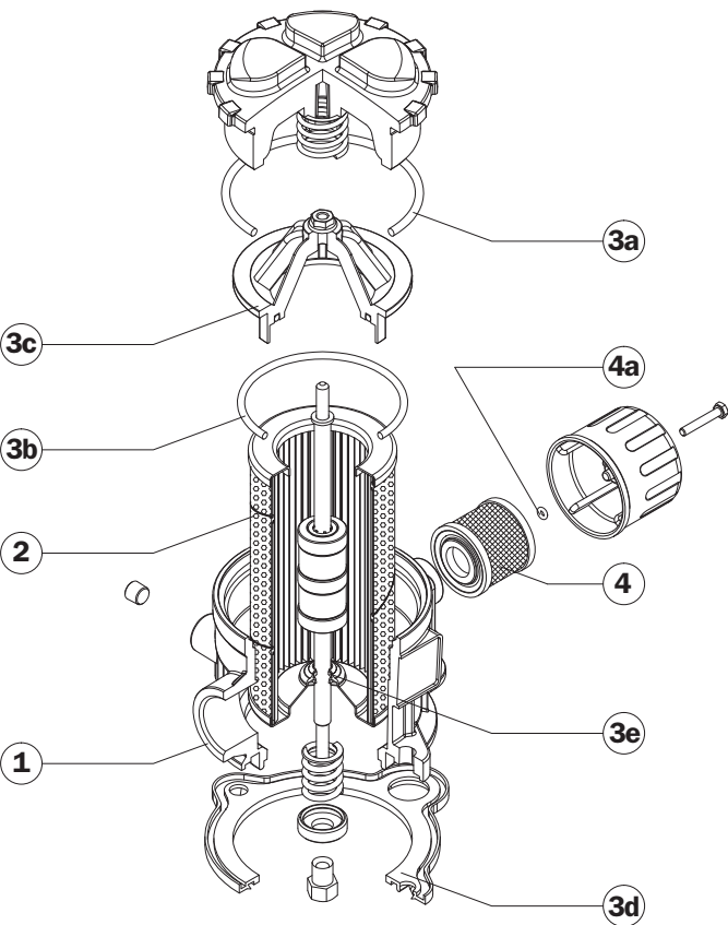
MPH 100 CO
